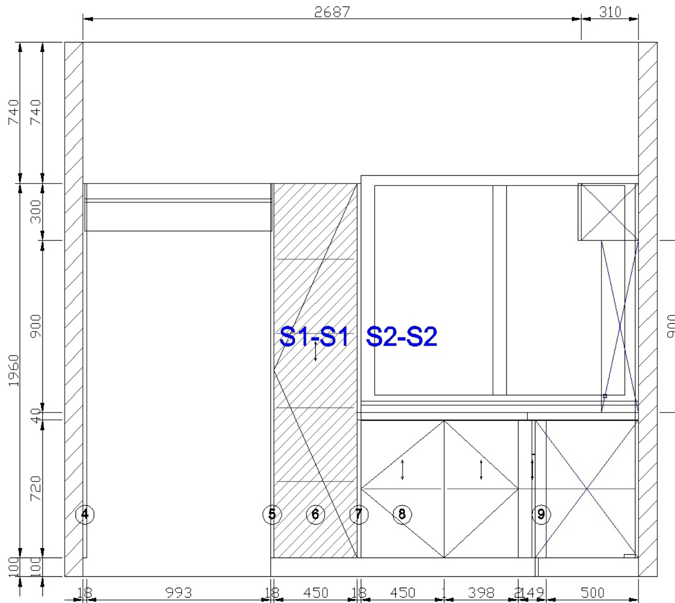
C View elevation drawing
