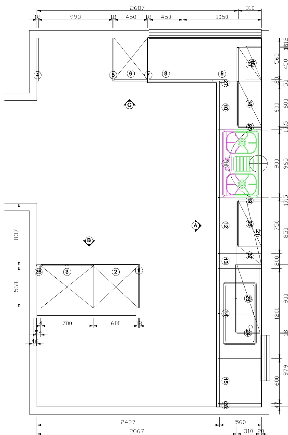
Plan drawing
