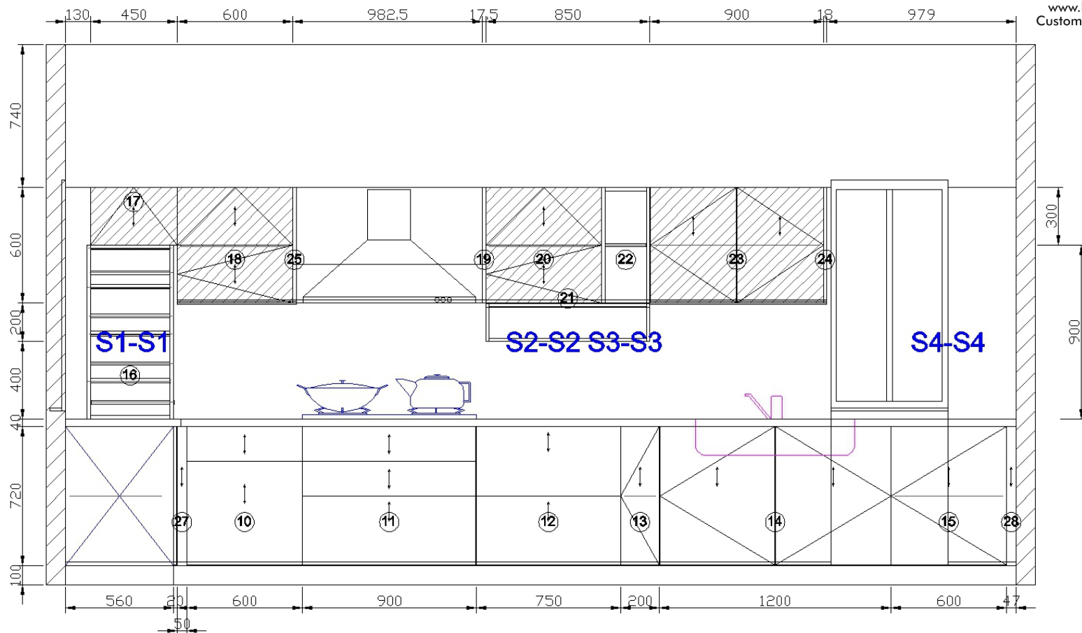
A View elevation drawing
